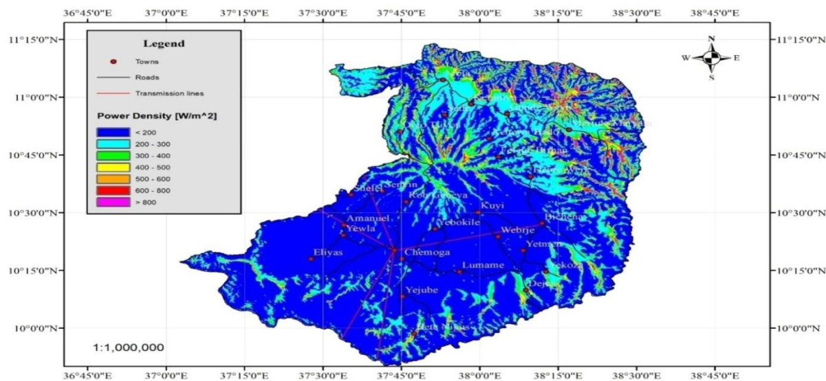
Figure 8. East Gojjam Zone power density map at 50 m.
